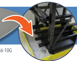
Acid pillows at bottom of battery rack
